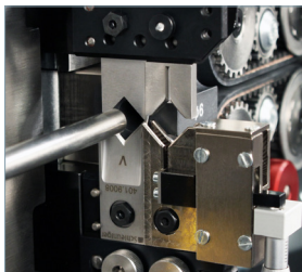
Indexing cutter head and SmartBlade™ system with cartridges and libraries for quick changeover of complete blade sets
